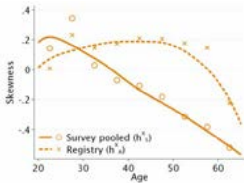
(c) Skewness
